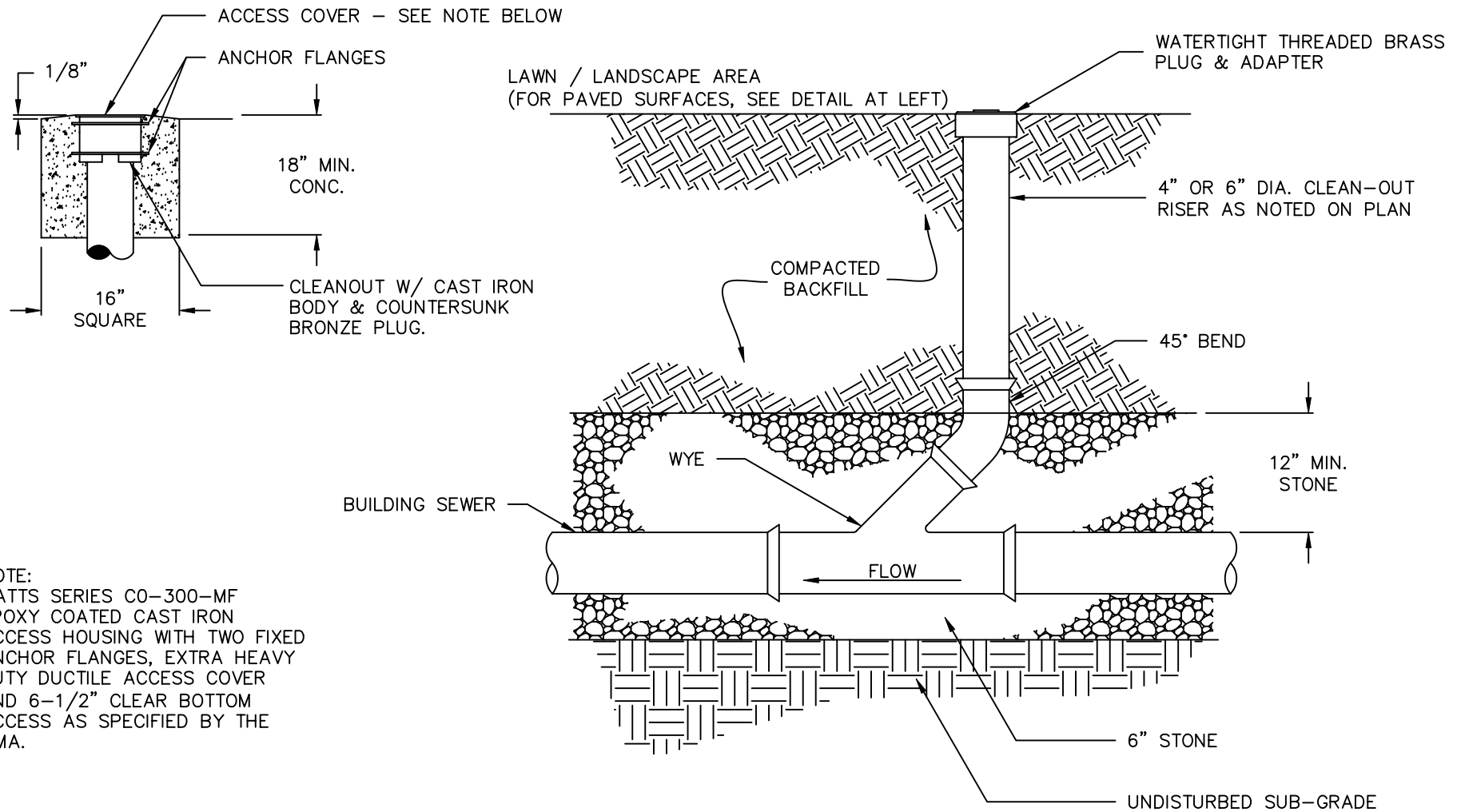
BUILDING SEWER CLEAN-OUT DETAIL
