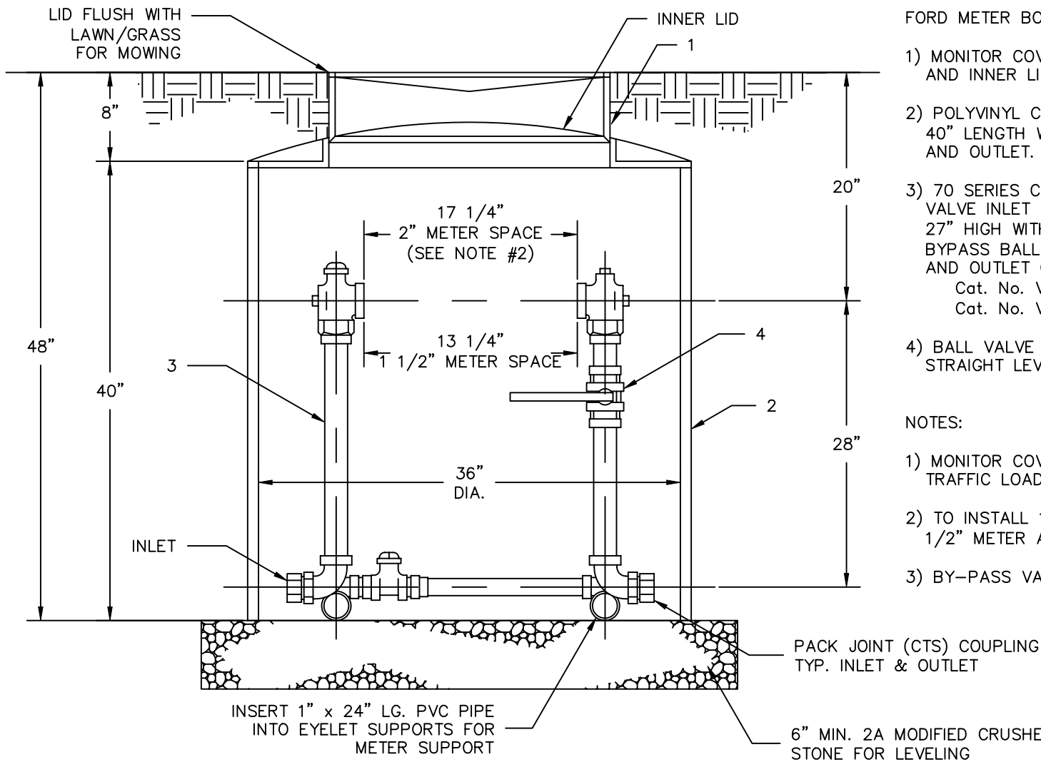
METER PIT ASSEMBLY FOR 1 1/2" AND 2" WATER METERS
